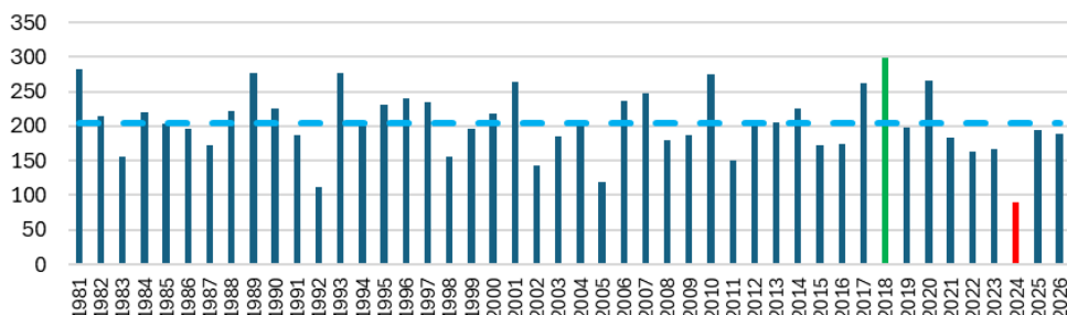
Zambia Average Total Rainfall for February (mm)
