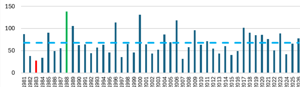
South Africa Average Total Rainfall for February (mm)
