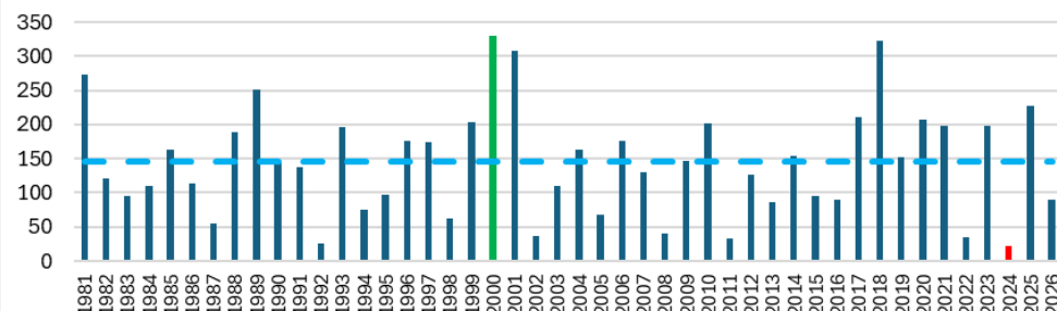
Zimbabwe Average Total Rainfall for February (mm)
