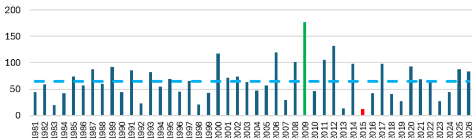
Namibia Average Total Rainfall for February (mm)
